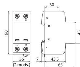
Dimension drawing DSH TN 255
