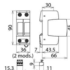
Dimension drawing DG M TN 275 FM
