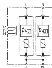
Basic circuit diagram DG M TN 275 FM
