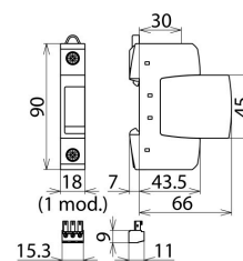
Dimension drawing DG S 275 FM
