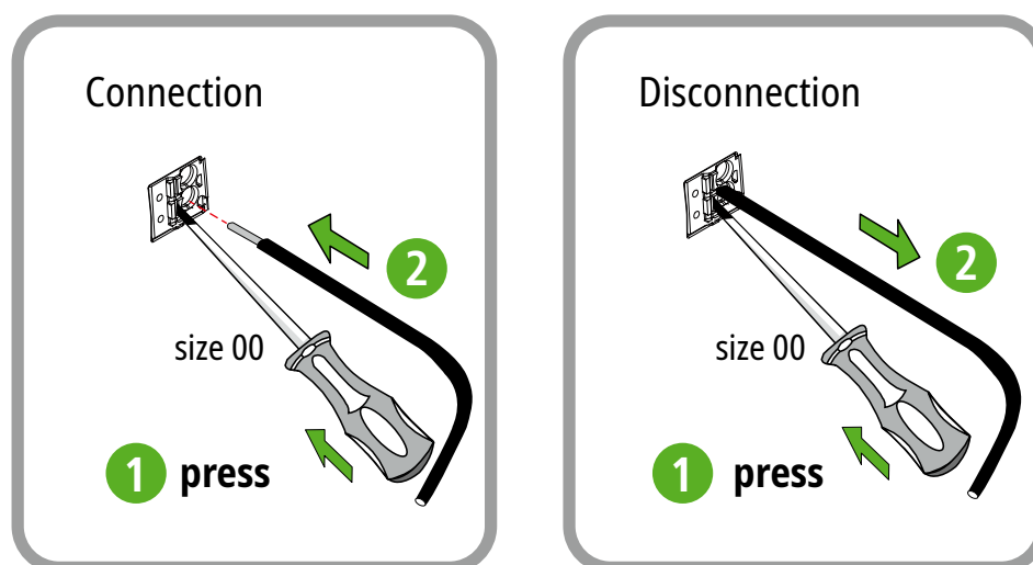
Fig. 3.4 Connection or disconnection
