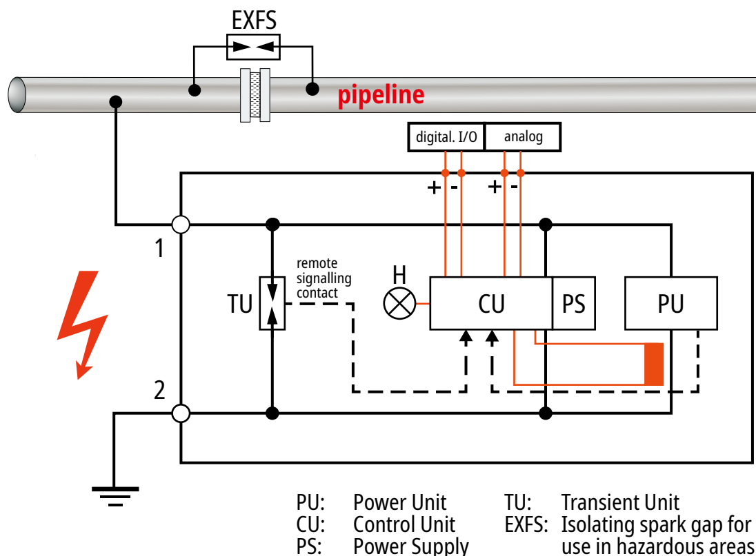
Fig. 2.2 Functional units
