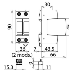
Dimension drawing DG M TT 2P 275 FM
