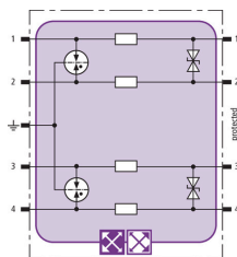
Basic circuit diagram BXT ML4 BD 60
