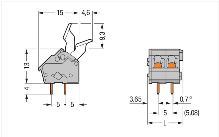
Dimensions in mm L = (pole no. x pin spacing) + 2.9 mm For lengths greater than three poles, finger lever operation for center levers may not be possible due to finger size/spacing limitations.
