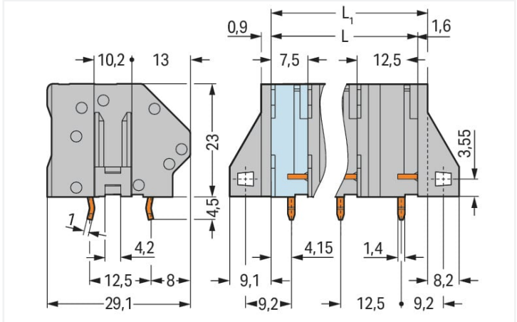
Dimensions in mm L = (pole no. – 1) x pin spacing + 7.5 mm L1 = L + 1.6 mm ± version without mounting flange
