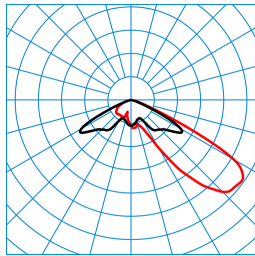
LnPlus 70-AM19L/42000-730 36G1 ETDD (CLO end value) TX377338
