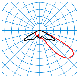
LnPlus 70-AM19L/42000-730 36G1 ETDD (CLO initial value) TX377060
