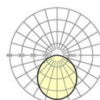
HLAG/1200 LED 2400 lm 840
