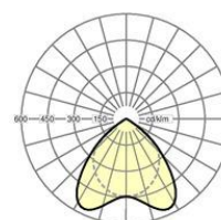
CUHX/1200-1 LED 3400 lm 840
