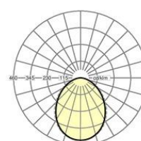
PREG/300-1200 IP54 LED 4700 lm 840
