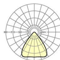
WOHTB/1300 IP54 LED 29200 lm 840
