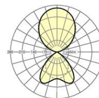
SHXI/1500-2 LED 6800 lm 840
