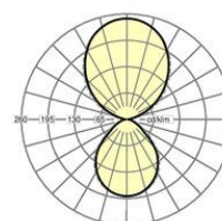
SHPI/1500-2 LED 6700 lm 840
