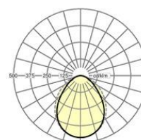
RSAGHC-1500 LED 3200 lm 840
