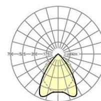
RSEX/300 -1200 LED 3100 lm 840
