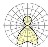
SHLXI/1200-2 LED 5500 lm 840
