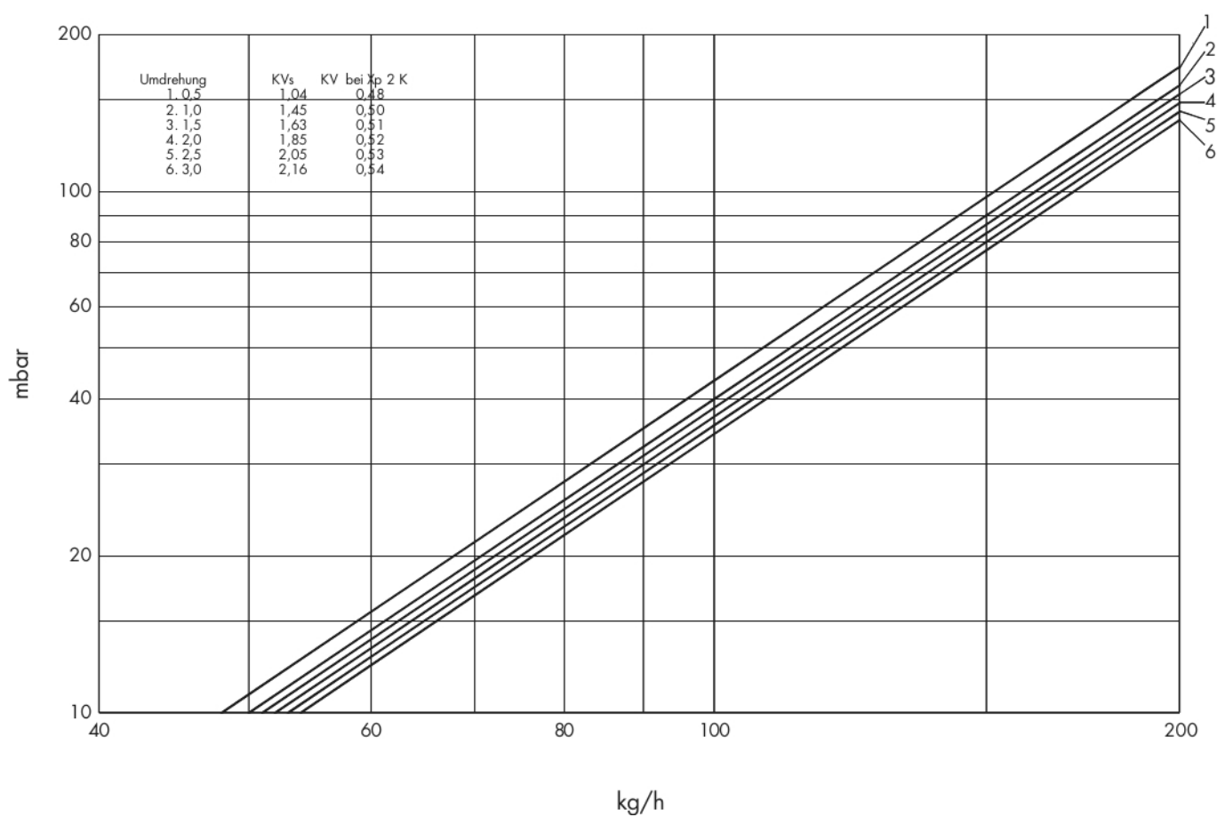
Thermostatventil Eckform Eurokonus 2904123401 / 29041234##
