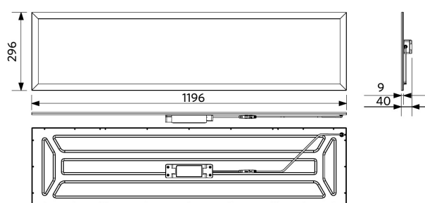
LEDPanelRc-S5 Driver Tunable White
