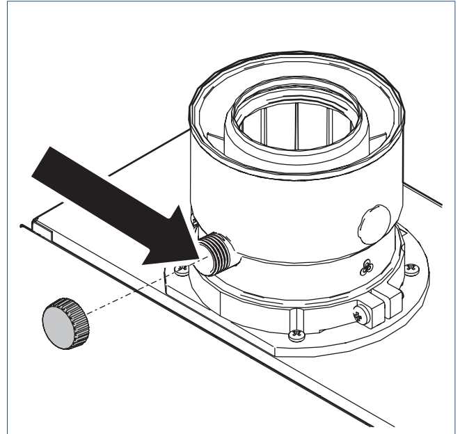
Meetnippeldop rookgasadapter.
