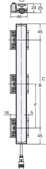
Mounting screw holes
