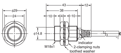
Fig. ⑥ E2AG-M18KN10-WS-B
