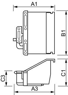
HID-STRAIN RELIEF
