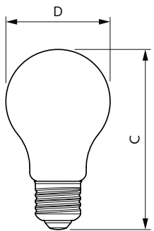
A60 230V 9-60W 806lm 2700K E27 D CL
