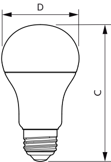
Bulb 220-240V 13-W 152lm 3000K E27 ND
