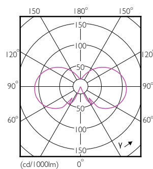
Light Distribution Diagram - CorePro LEDBulbND 4.3-40W E27 A60840 CLG
