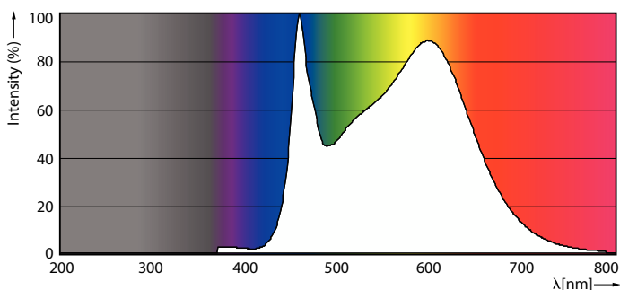
Spectral Power Distribution Colour - CorePro LEDBulbND 4.3-40W E27 A60840 CLG
