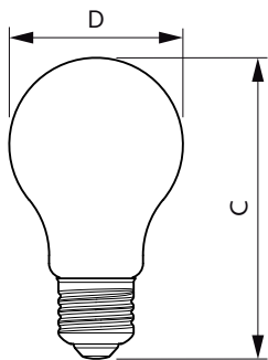
CorePro LEDBulbND 7-60W E27 A60 840 CL G
