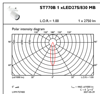
OFPC1_ST770B1xLED27S830MB
