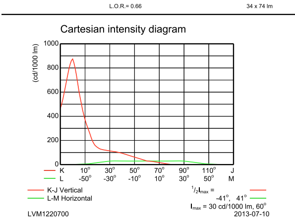
BBP623 GC 34xLED-HB/RD A
