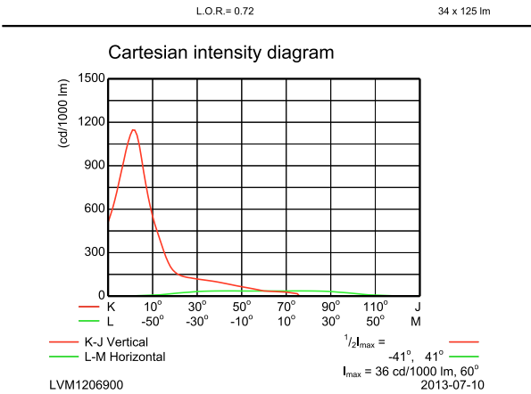
BBP623 GC 34xLED-HB/NW A
