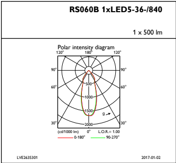
IFPC1_RS060B1xLED5-36-840
